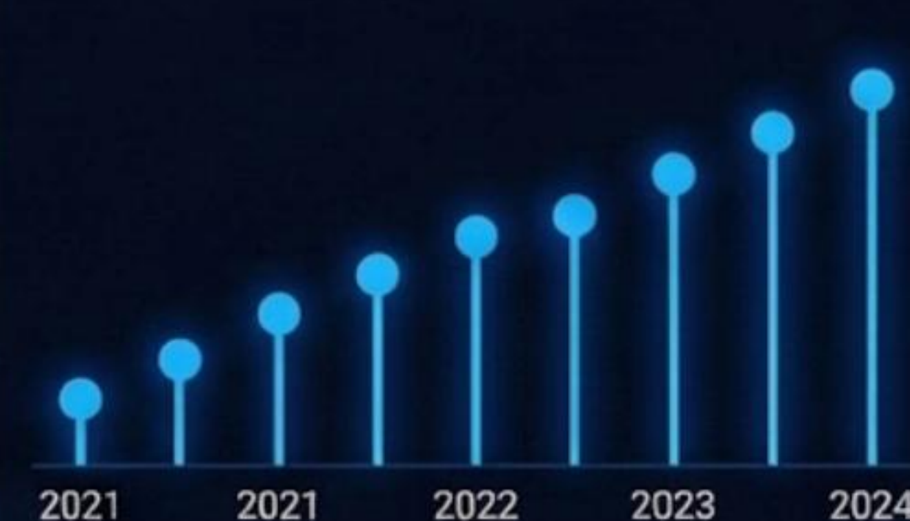
GWP Growth Lollipop Chart
